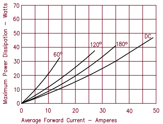
Figure 4 Maximum Forward Power Dissipation – Standard Polarity
