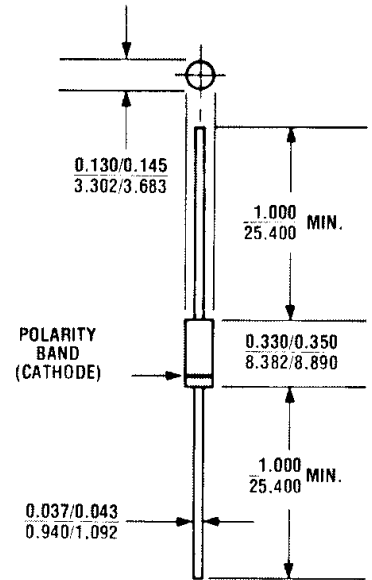
FIGURE 1 All dimensions in \frac{\text{INCH}}{\text{m.m.}}
