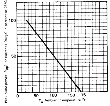
FIG. 3. Derating curve
