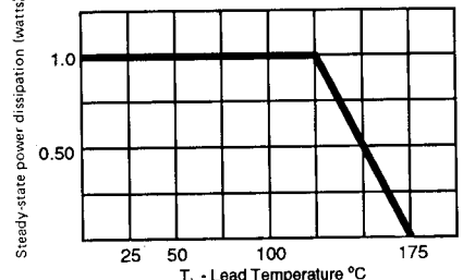
FIG. 4. Steady-state power derating curve
