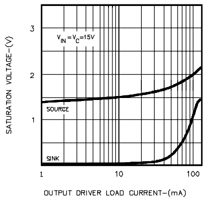
FIGURE 17. OUTPUT DRIVER SATURATION VOLTAGE
