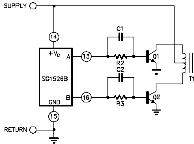
FIGURE 26. PUSH-PULL CONFIGURATION
