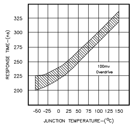
FIGURE 9. COMPARATOR INPUT TO DRIVER OUTPUT DELAY
