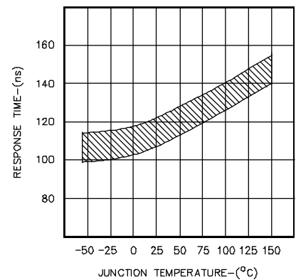
FIGURE 18. SHUTDOWN INPUT TO DRIVER OUTPUT DELAY
