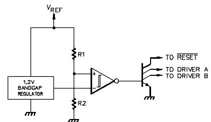
FIGURE 21. SIMPLIFIED UNDERVOLTAGE LOCKOUT
