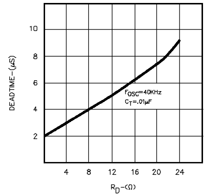
FIGURE 12. OUTPUT DRIVER DEADTIME VS. R_D VALUE
