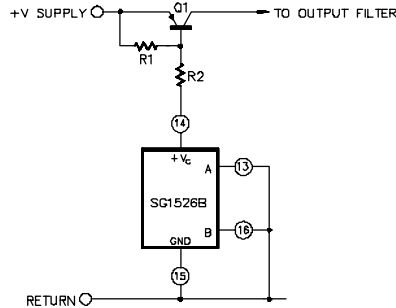
FIGURE 27. SINGLE-ENDED CONFIGURATION
