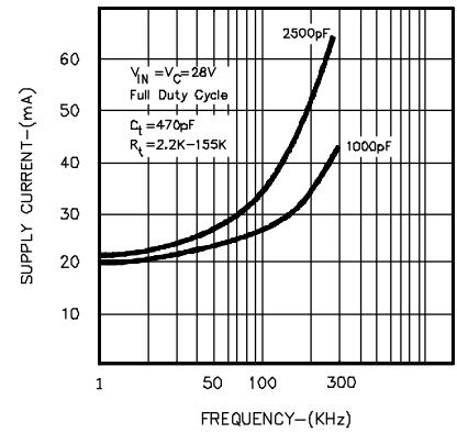
FIGURE 15. SUPPLY CURRENT VS. OUTPUT FREQUENCY
