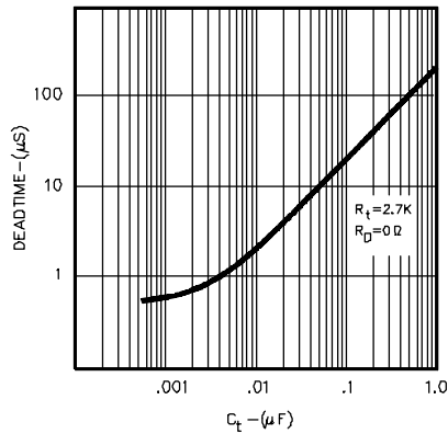
FIGURE 11. OUTPUT DRIVER DEADTIME VS. C_T VALUE
