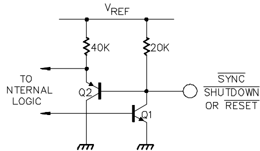
FIGURE 23 DIGITAL CONTROL PORT SCHEMATIC
