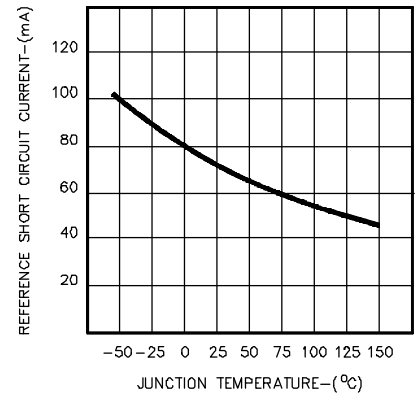
FIGURE 3. REFERENCE SHORT CIRCUIT
