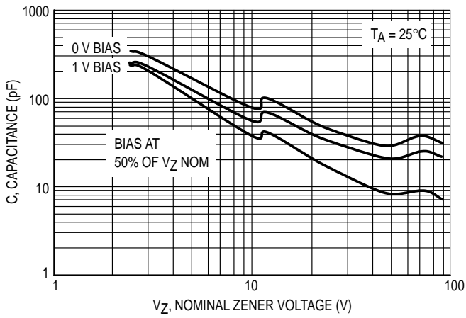
Figure 5. Typical Capacitance
