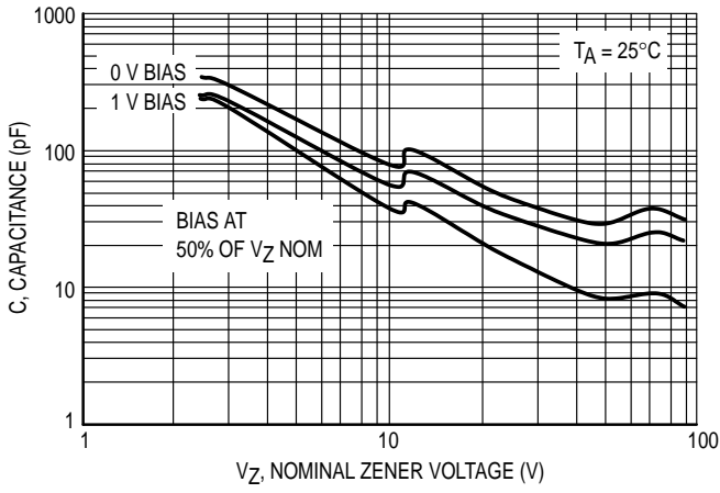
Figure 7. Typical Capacitance
