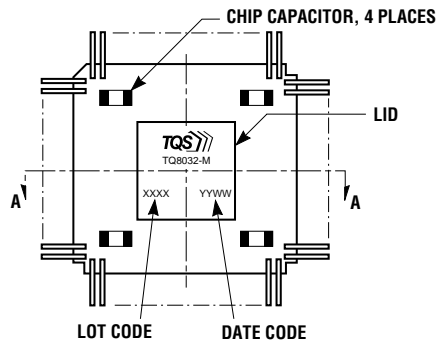
Figure 7. Mechanical Dimensions
