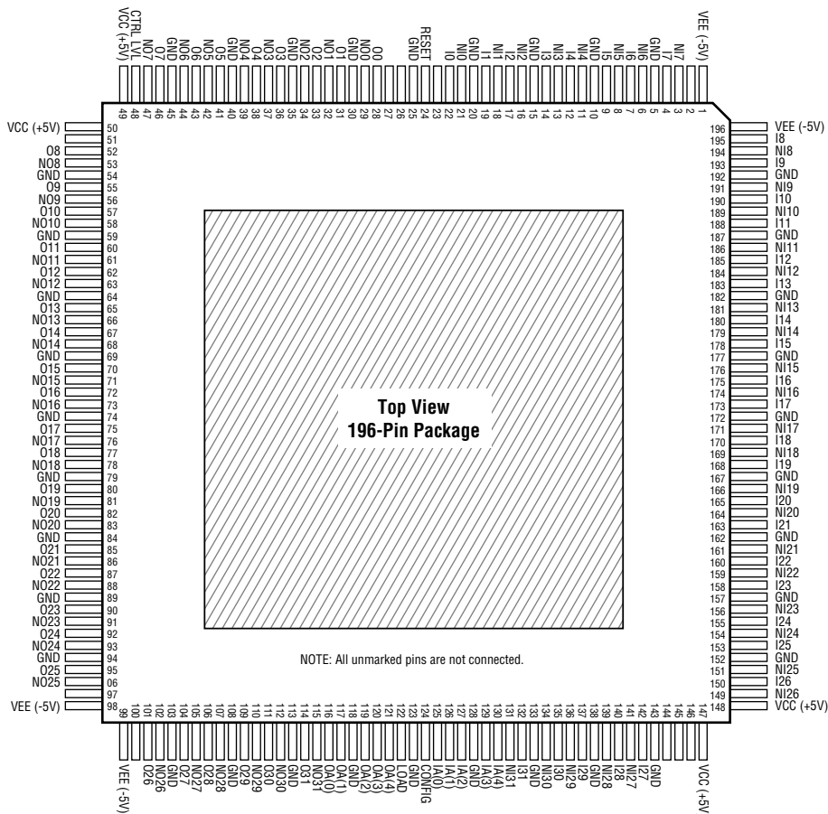
Figure 2. Package Pinout
