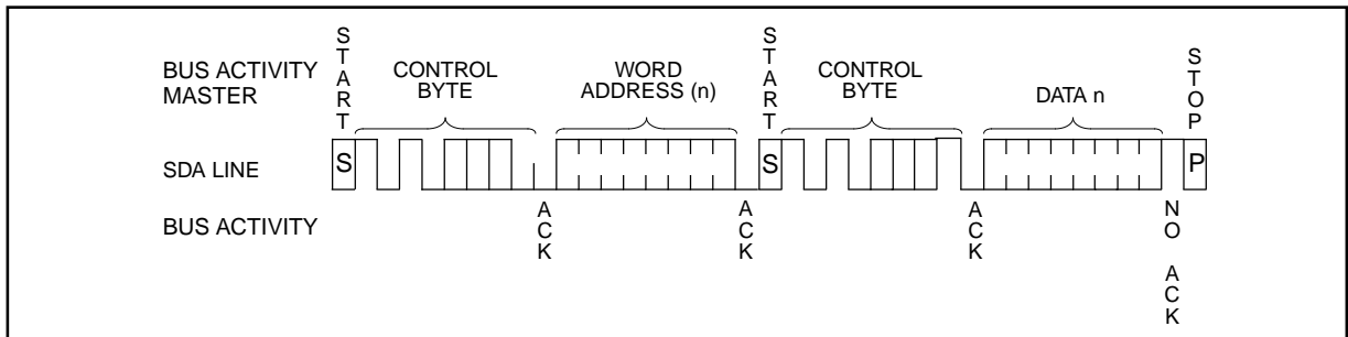
FIGURE 7-1: RANDOM READ
