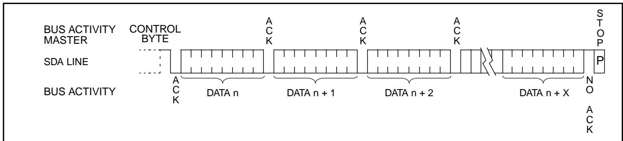
FIGURE 7-2: SEQUENTIAL READ
