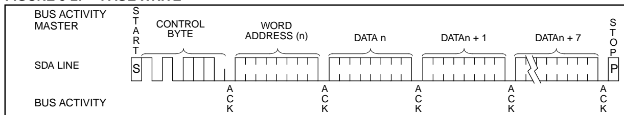
FIGURE 5-2: PAGE WRITE
