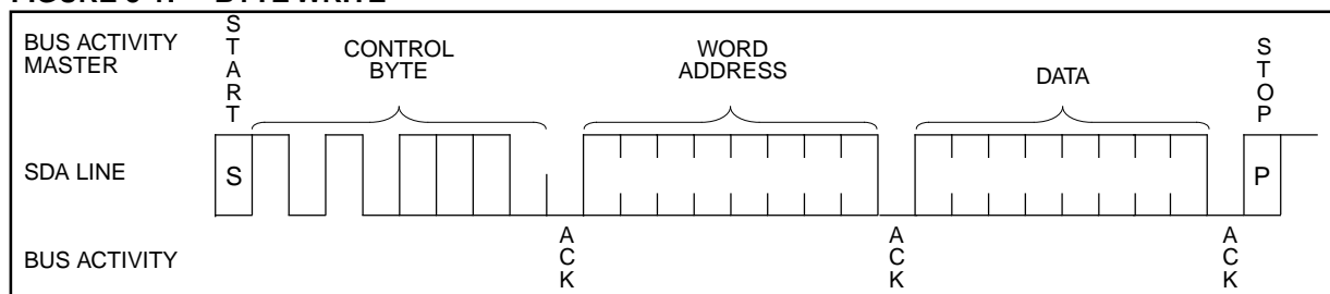
FIGURE 5-1: BYTE WRITE
