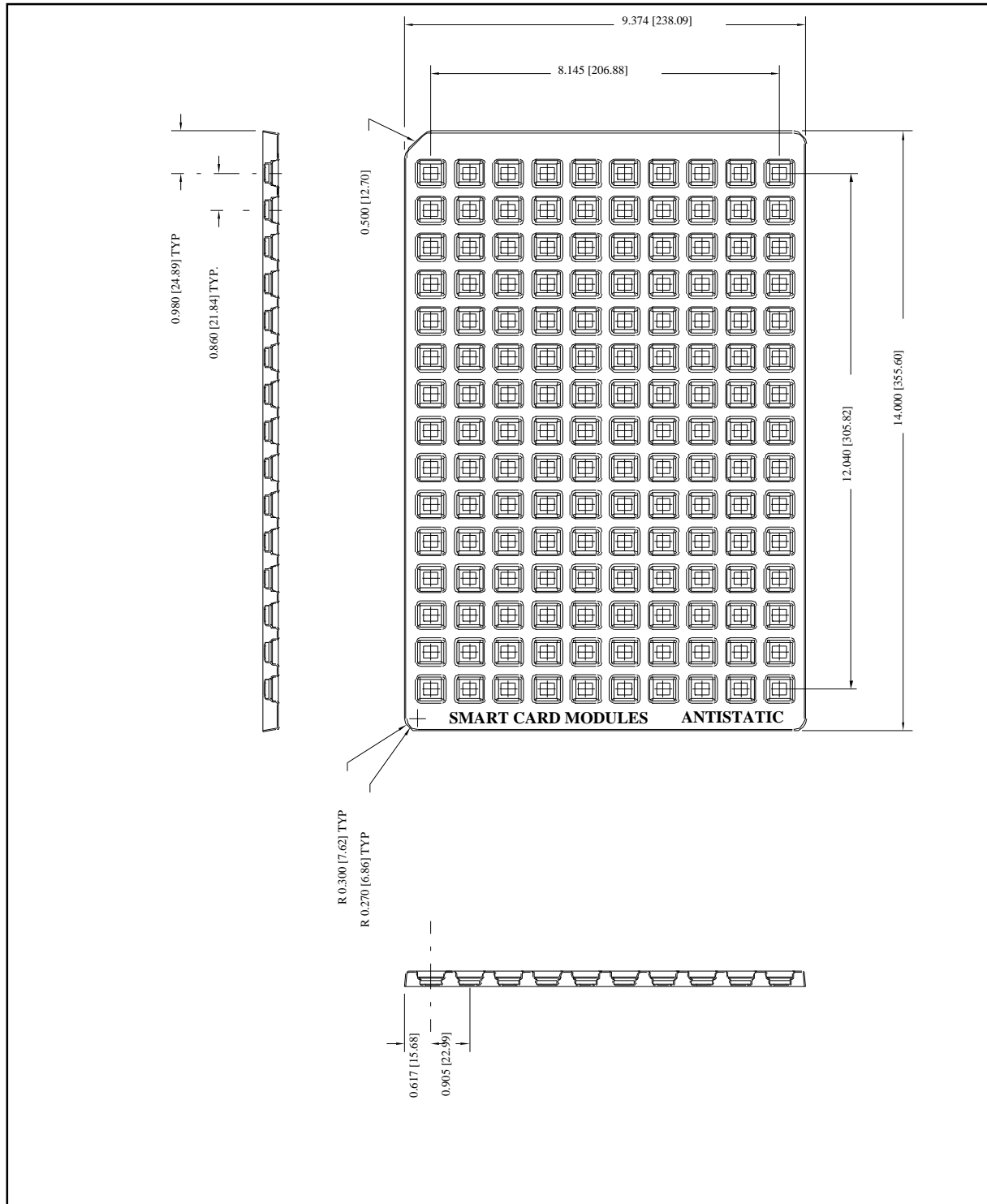
FIGURE 8-1: TRAY DIMENSIONS
