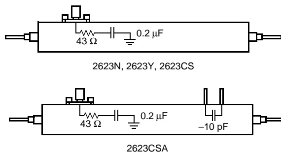
Figure 2. Equivalent Circuit Diagram
