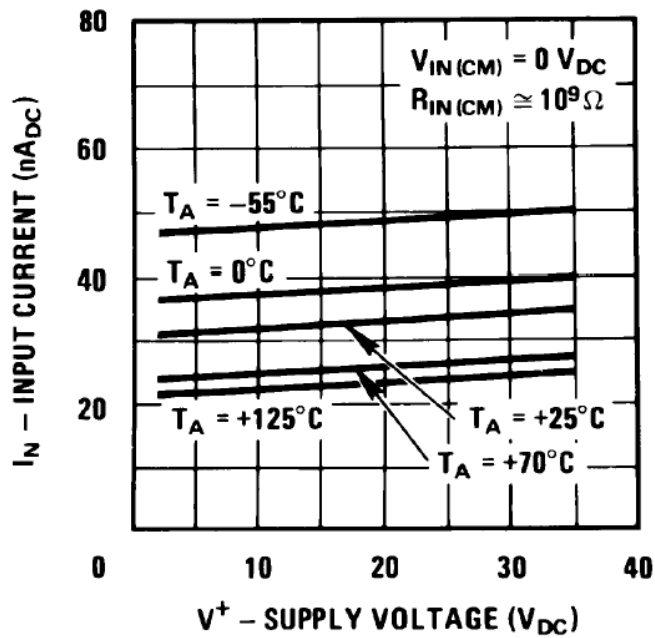
FIGURE 2. INPUT CURRENT
