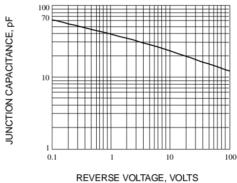
Fig. 3-TYPICAL JUNCTION CAPACITANCE
