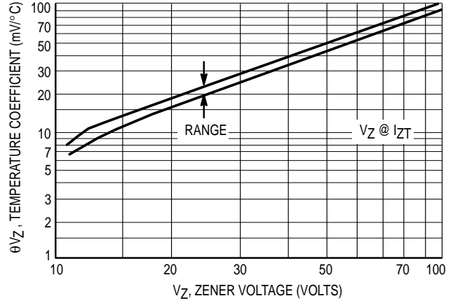
Figure 2. Temperature Coefficients
