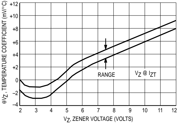
Figure 2. Temperature Coefficients
