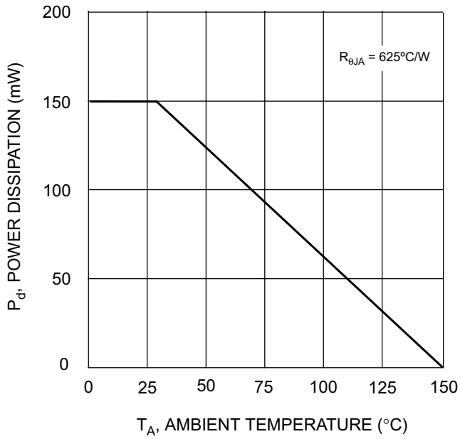
Fig. 1 Derating Curve
