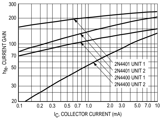
Figure 11. Current Gain
