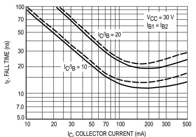
Figure 8. Fall Time
