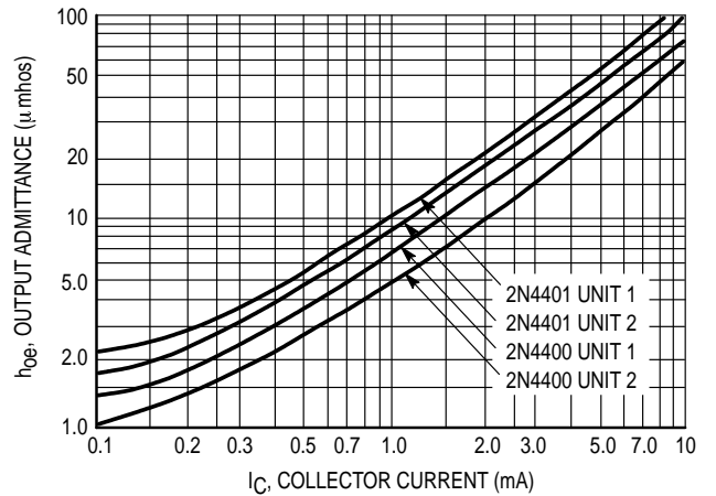
Figure 14. Output Admittance
