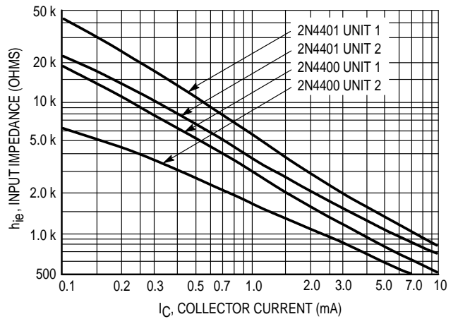
Figure 12. Input Impedance
