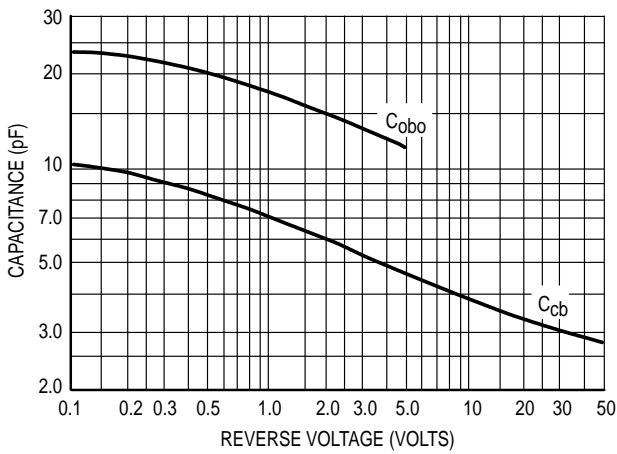
Figure 3. Capacitances
