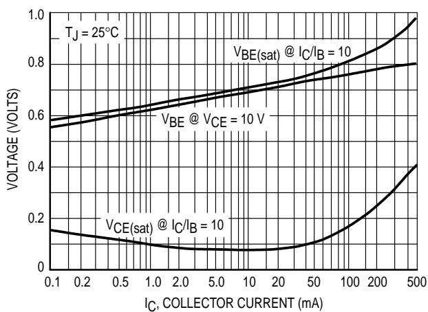
Figure 17. "On" Voltages
