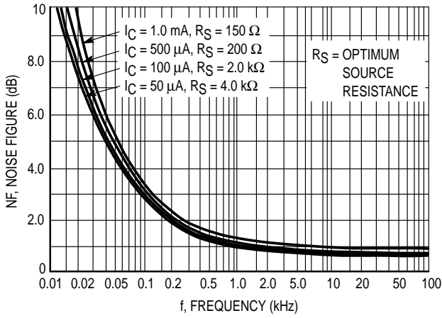
Figure 9. Frequency Effects
