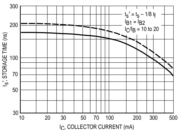
Figure 7. Storage Time
