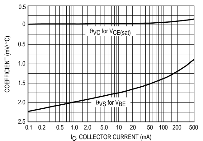
Figure 17. Temperature Coefficients
