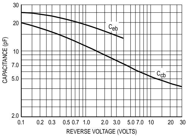
Figure 3. Capacitances
