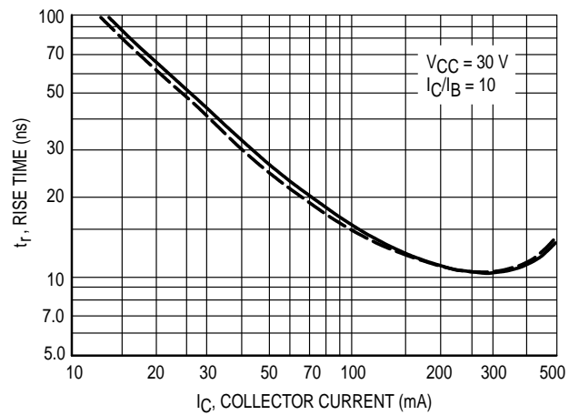
Figure 6. Rise Time
