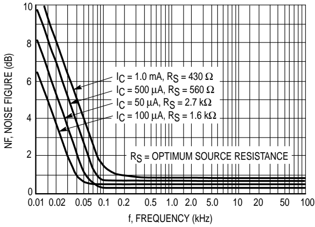
Figure 8. Frequency Effects
