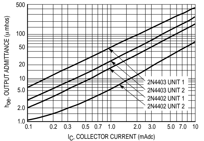
Figure 13. Output Admittance
