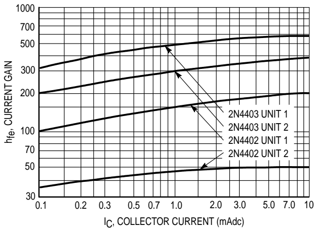
Figure 10. Current Gain
