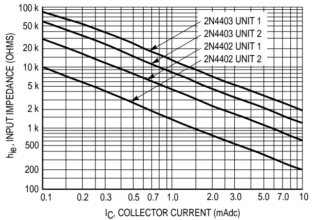
Figure 11. Input Impedance
