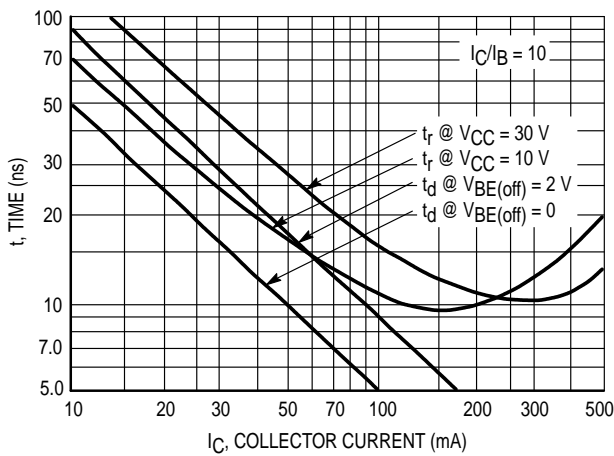
Figure 5. Turn-On Time
