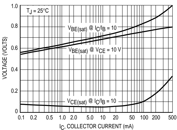
Figure 16. "On" Voltages
