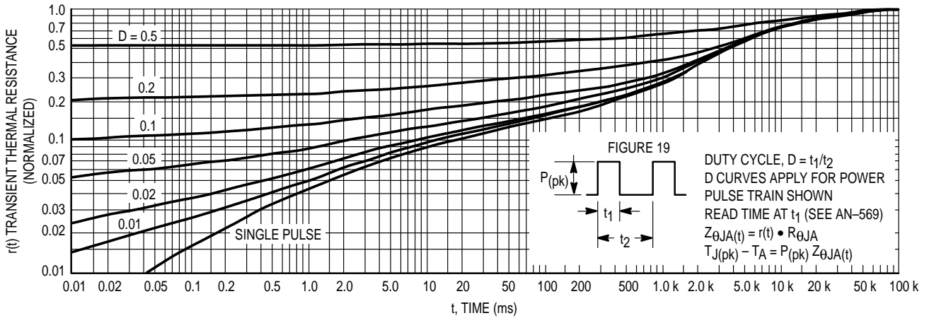
Figure 17. Thermal Response
