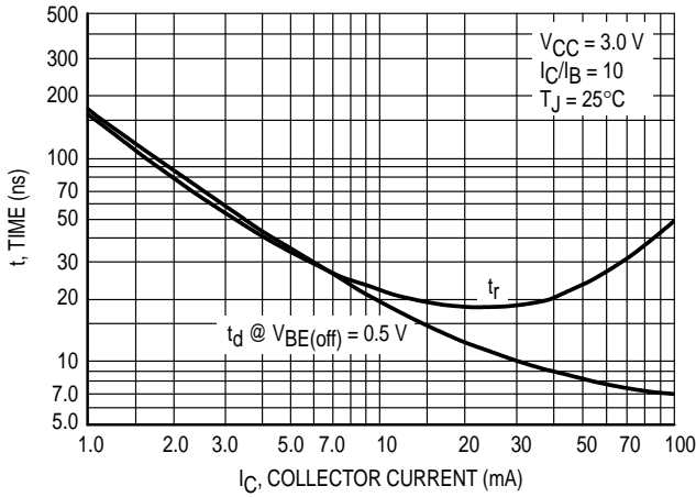
Figure 11. Turn-On Time
