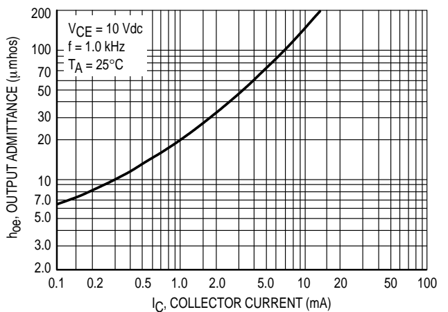
Figure 16. Output Admittance
