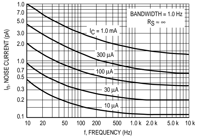
Figure 2. Noise Current
