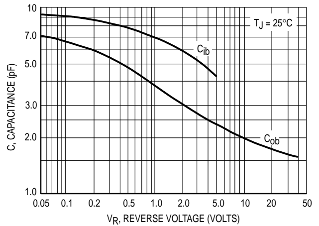
Figure 14. Capacitance
