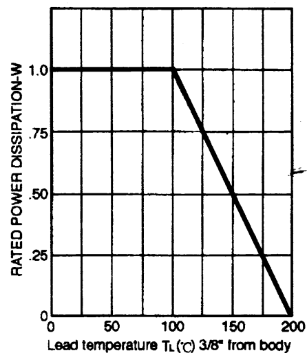
FIGURE 5 POWER DERATING CURVE
