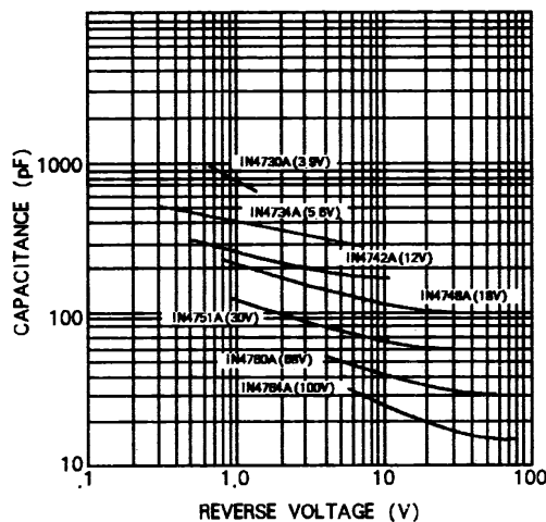
FIGURE 2 CAPACITANCE vs. VOLTAGE FOR REPRESENTATIVE TYPES
