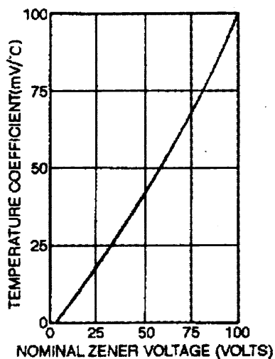
FIGURE 4 TEMP. COEFF. vs. ZENER VOLTAGE
