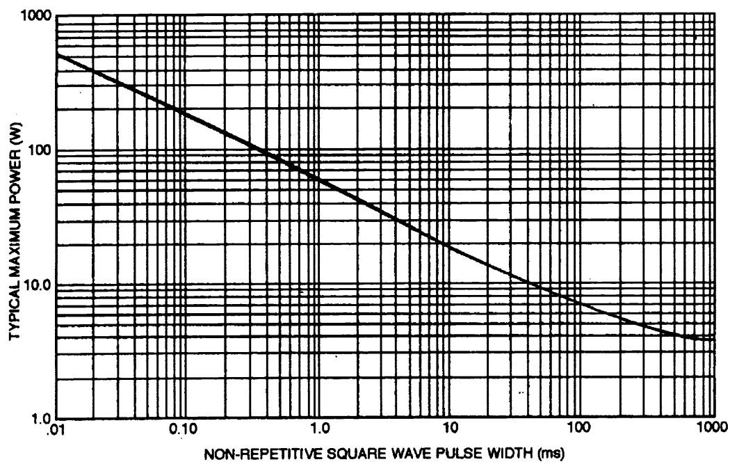
FIGURE 2 TRANSIENT SURGE CAPABILITY
