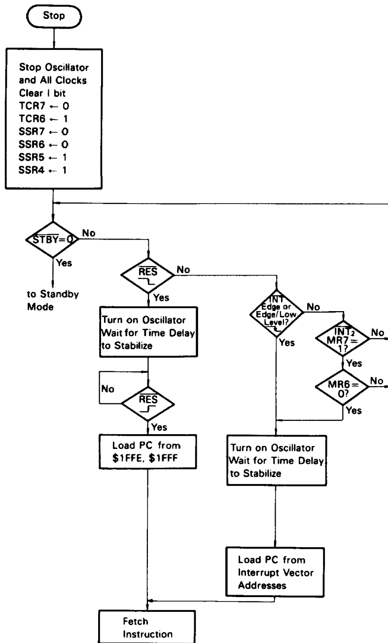
Figure 19 Stop Mode Flowchart
