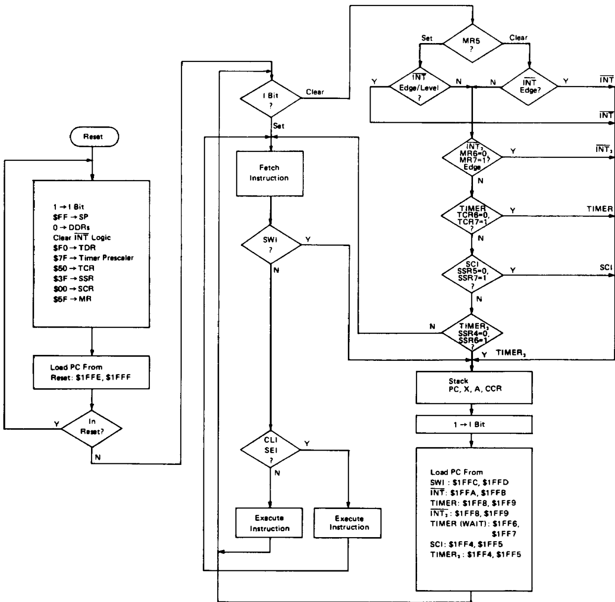
Figure 7 Interrupt Flowchart
