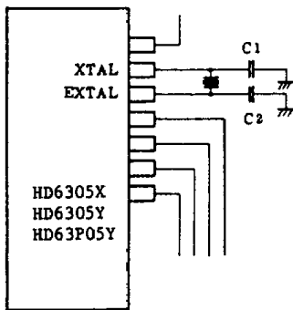
Figure 35 Design of Oscillation Circuit Board
