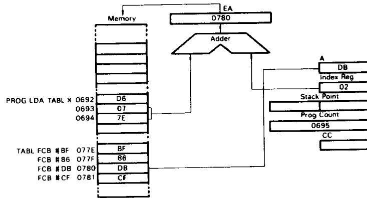
Figure 31 Example of Index (16-bit Offset) Addressing
