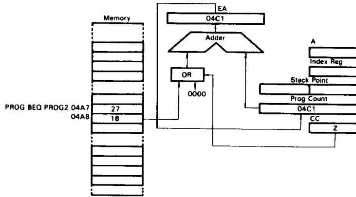
Figure 28 Example of Relative Addressing
