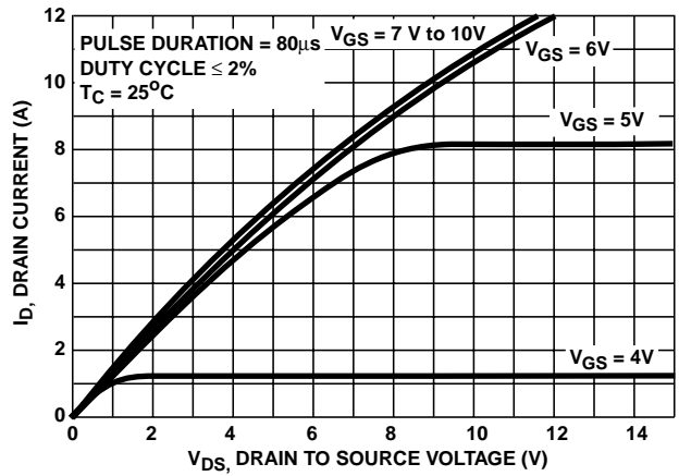
FIGURE 4. SATURATION CHARACTERISTICS
