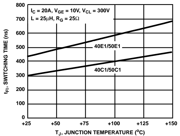
FIGURE 12. TYPICAL FALL TIME ( I_C = 20A )
