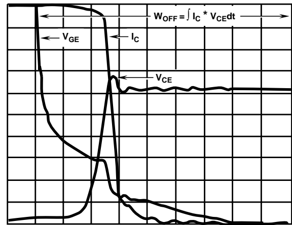
FIGURE 10. TYPICAL INDUCTIVE SWITCHING WAVEFORMS
