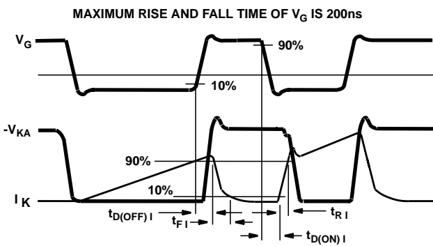
FIGURE 15. SWITCHING TEST WAVEFORMS
