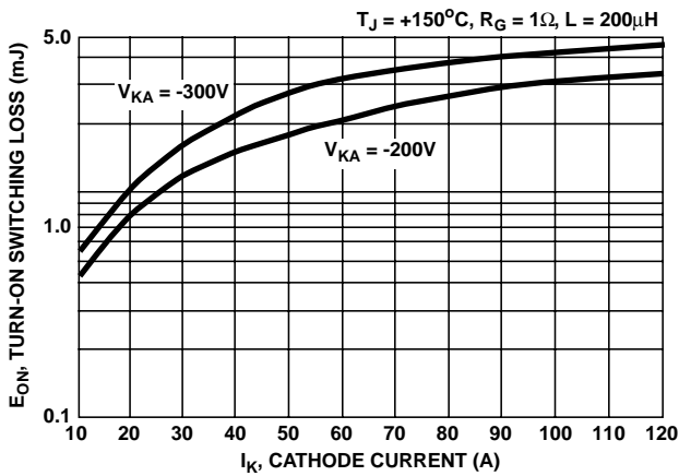
FIGURE 7. TURN-ON ENERGY LOSS vs CATHODE CURRENT (TYPICAL)
