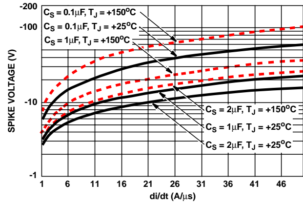
FIGURE 12. SPIKE VOLTAGE vs di/dt (TYPICAL)
