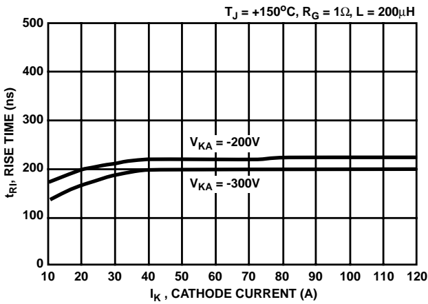
FIGURE 5. TURN-ON RISE TIME vs CATHODE CURRENT (TYPICAL)
