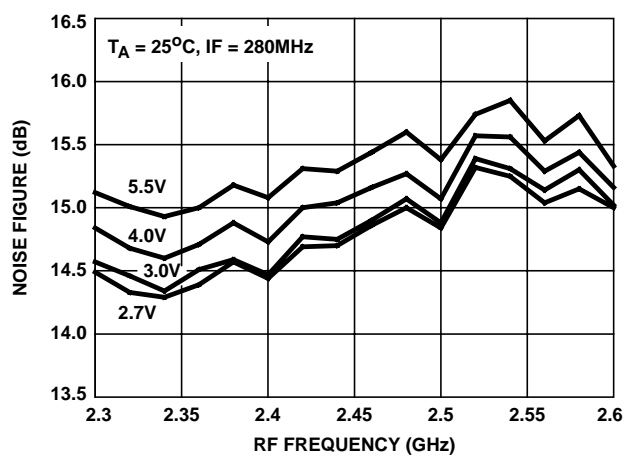
FIGURE 31. RECEIVE MIXER SSB NOISE FIGURE vs RF FREQUENCY
