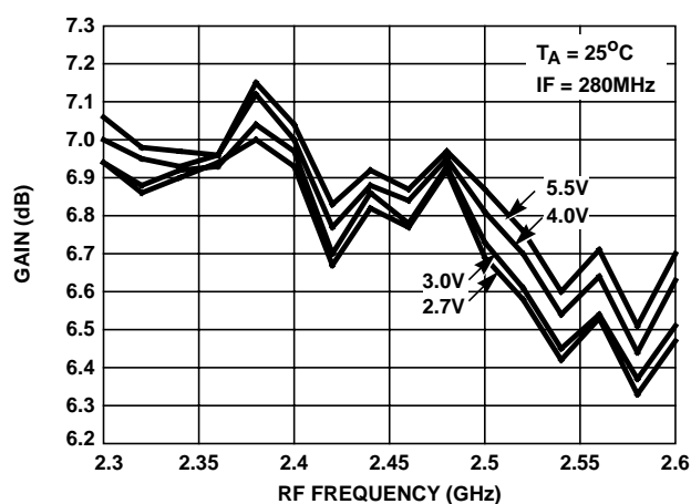
FIGURE 29. RECEIVE MIXER GAIN vs RF FREQUENCY FOR FIXED IF FREQUENCY
