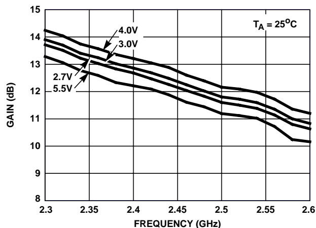
FIGURE 27. PRE-AMPLIFIER GAIN vs FREQUENCY
