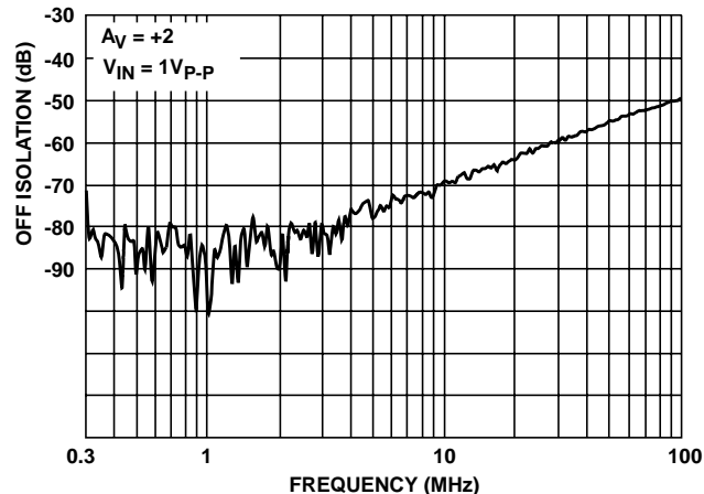
FIGURE 20. OFF ISOLATION
