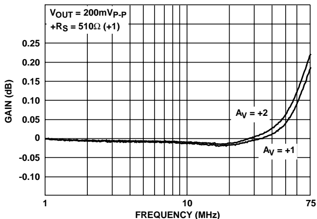
FIGURE 19. GAIN FLATNESS
