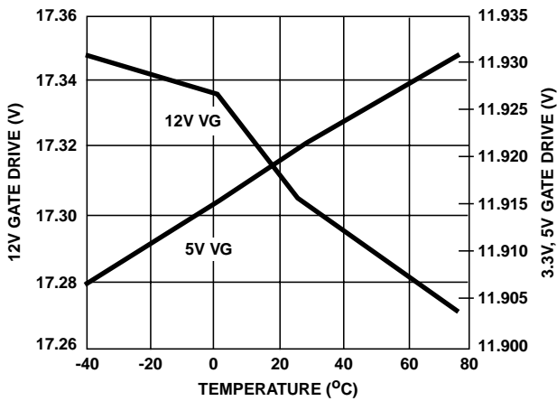
FIGURE 5. 12V, 5V GATE DRIVE
