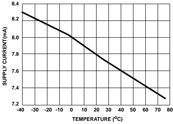
FIGURE 1. SUPPLY CURRENT
